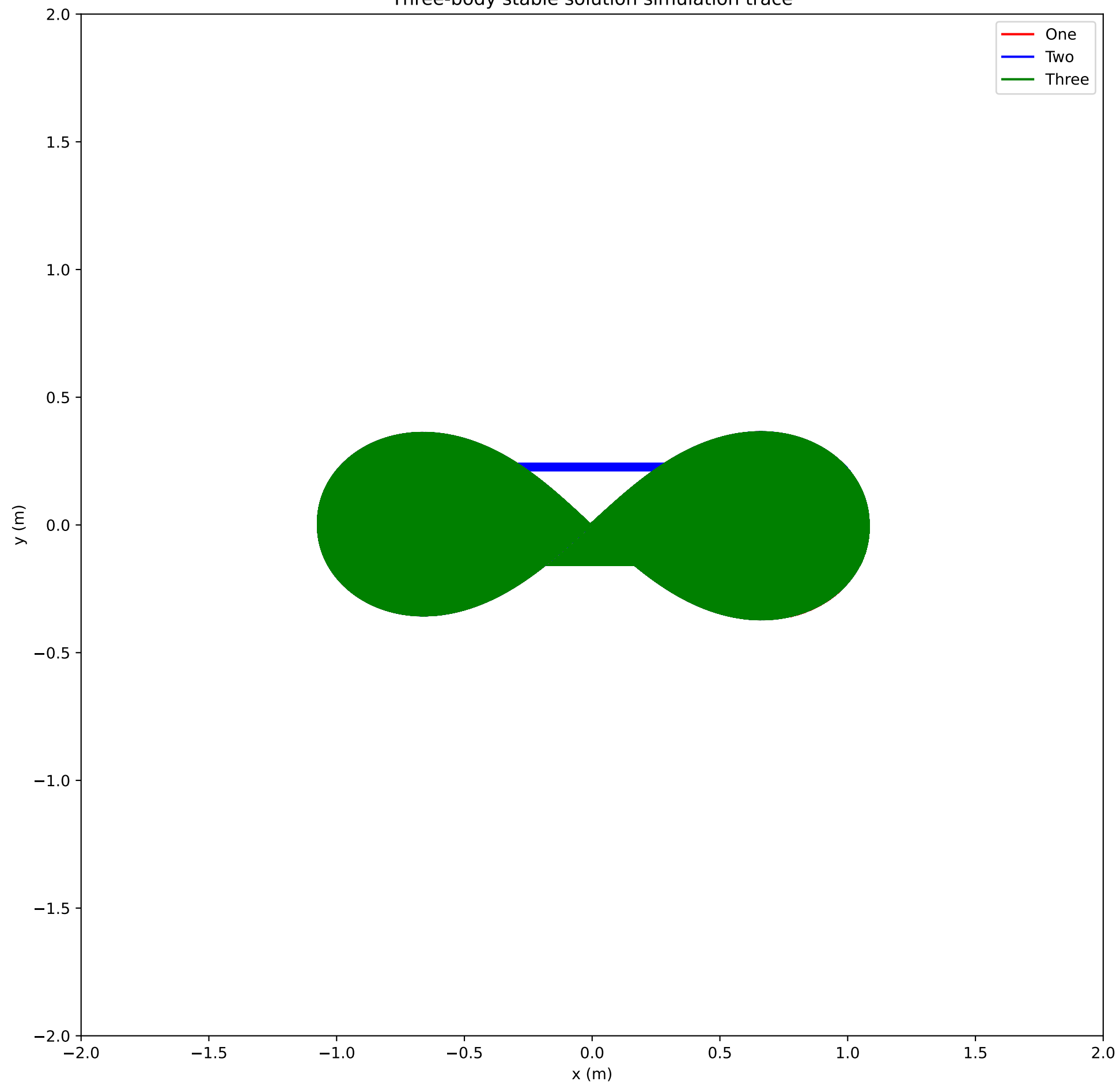
Three-body stable solution simulation trace
